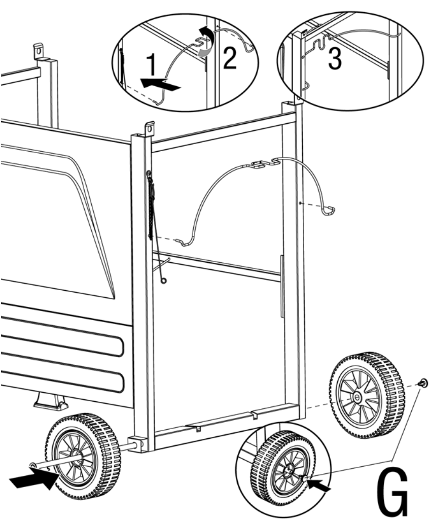
Attach LP Gas Tank Retainer Wire, Axle and Wheels
