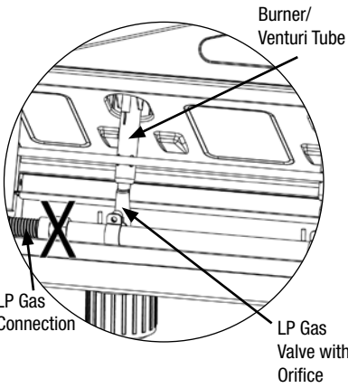
Figure 2: Side Burner
